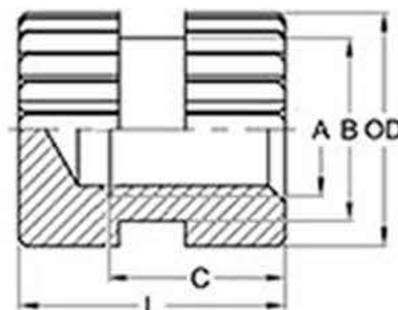
blind-hole
